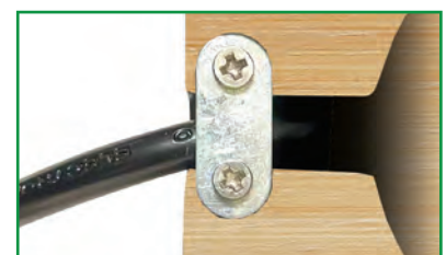
Anti-theft Cable Lock System
